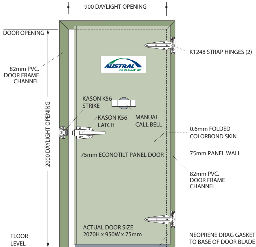
EXTERNAL ELEVATION
