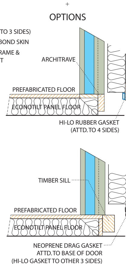
CROSS SECTIONS
