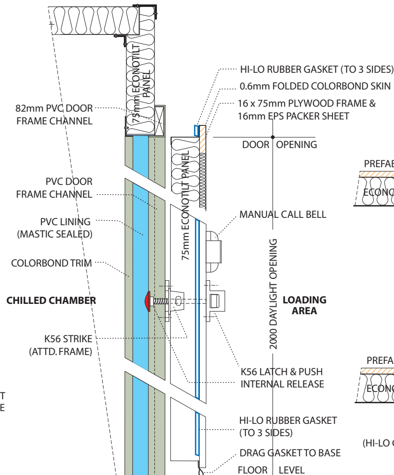
CROSS SECTIONS
