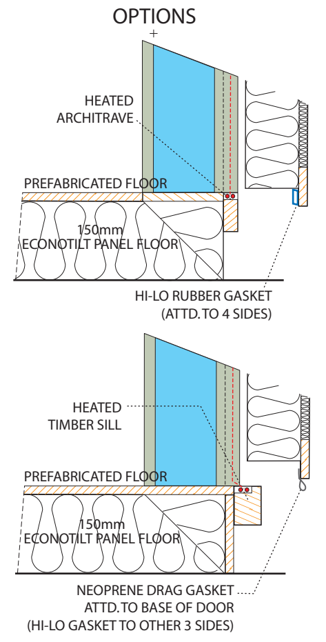
CROSS SECTIONS SCALE 1:10 Note: Plug doors shown open for clarity.
