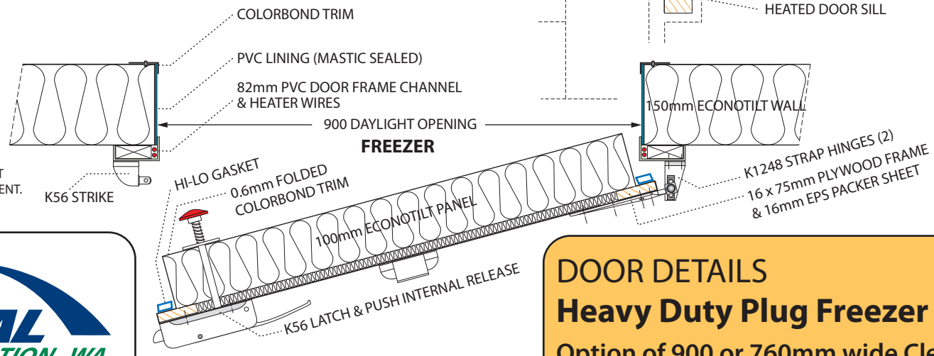
CROSS SECTIONS SCALE 1:10 Note: Plug doors shown open for clarity.
