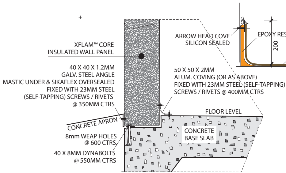
EXTERNAL WALL BASE
