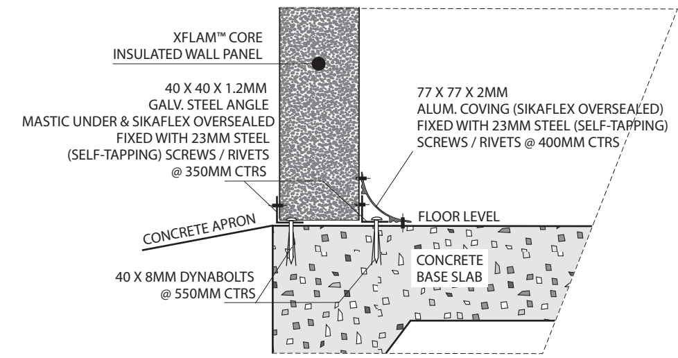
EXTERNAL WALL BASE
